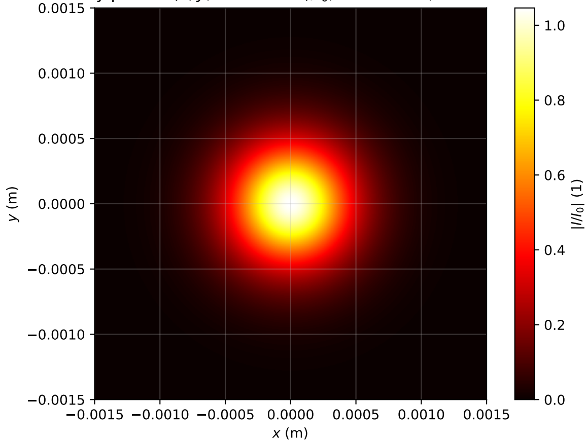
Intensity profile I(x, y, z = 1.035m)/I_0 , P_{in}=0.5P_{cr} , artificial time
